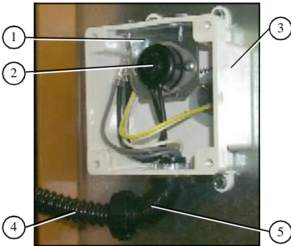
Lower plenum high limit thermostat.
